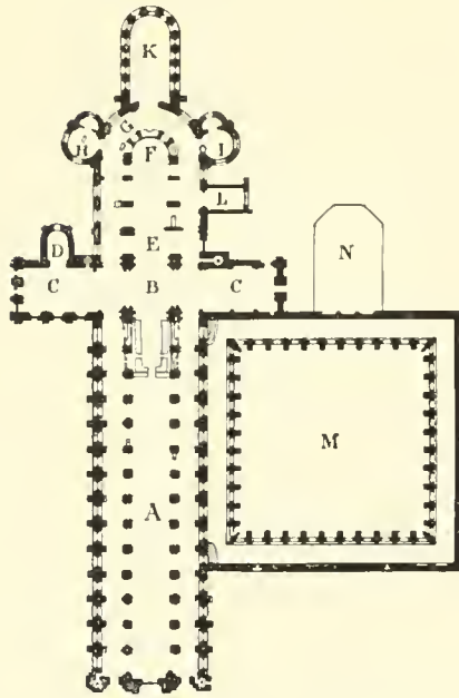
PLAN OF NORWICH CATHEDRAL. NORMAN STYLE.
